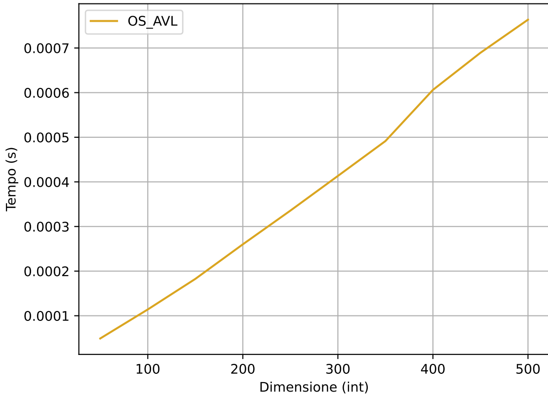
OS AVL - Test Casual Deletion
